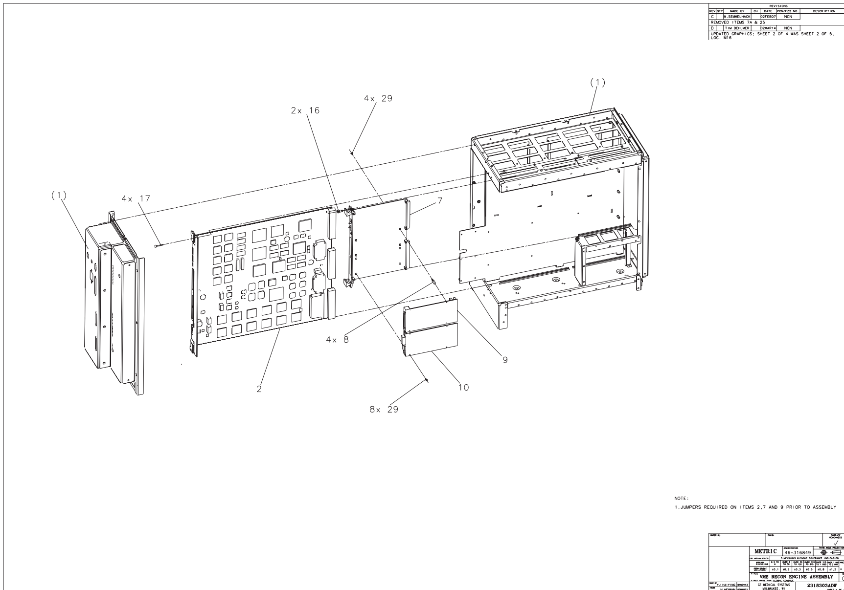
Figure 7-10 VME Recon Engine Assembly (2318303, sheet 2, rev 0)
