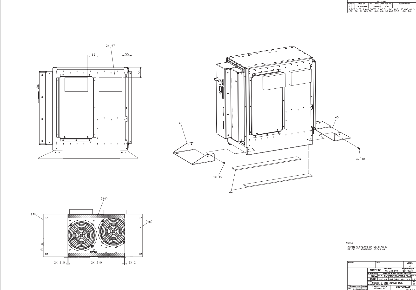
Figure 7-20 VME Chassis Assembly (2307794, sheet 3, rev 0)
