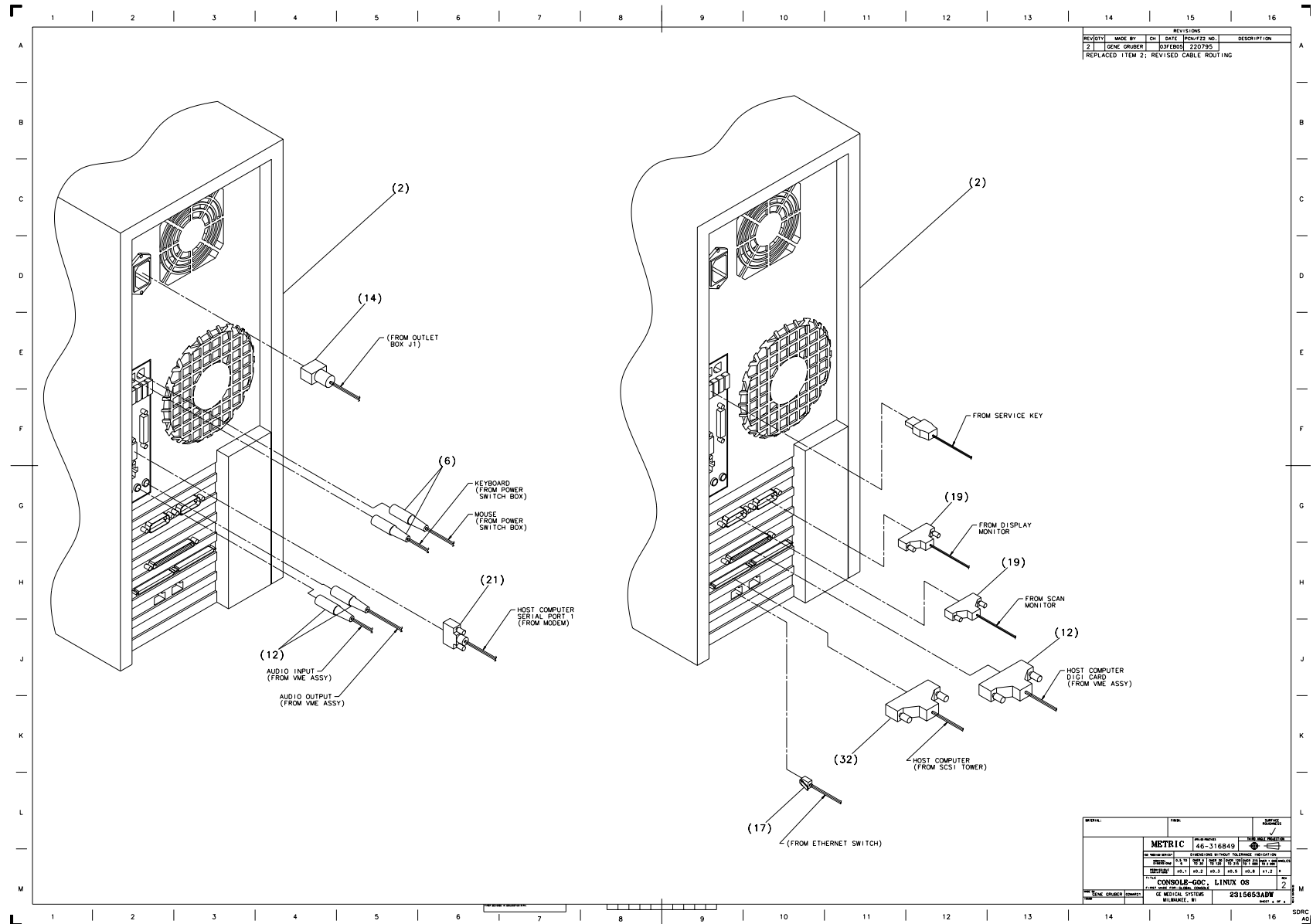
Figure 7-6 Console Assembly (2315653, sheet 4, rev 2)
