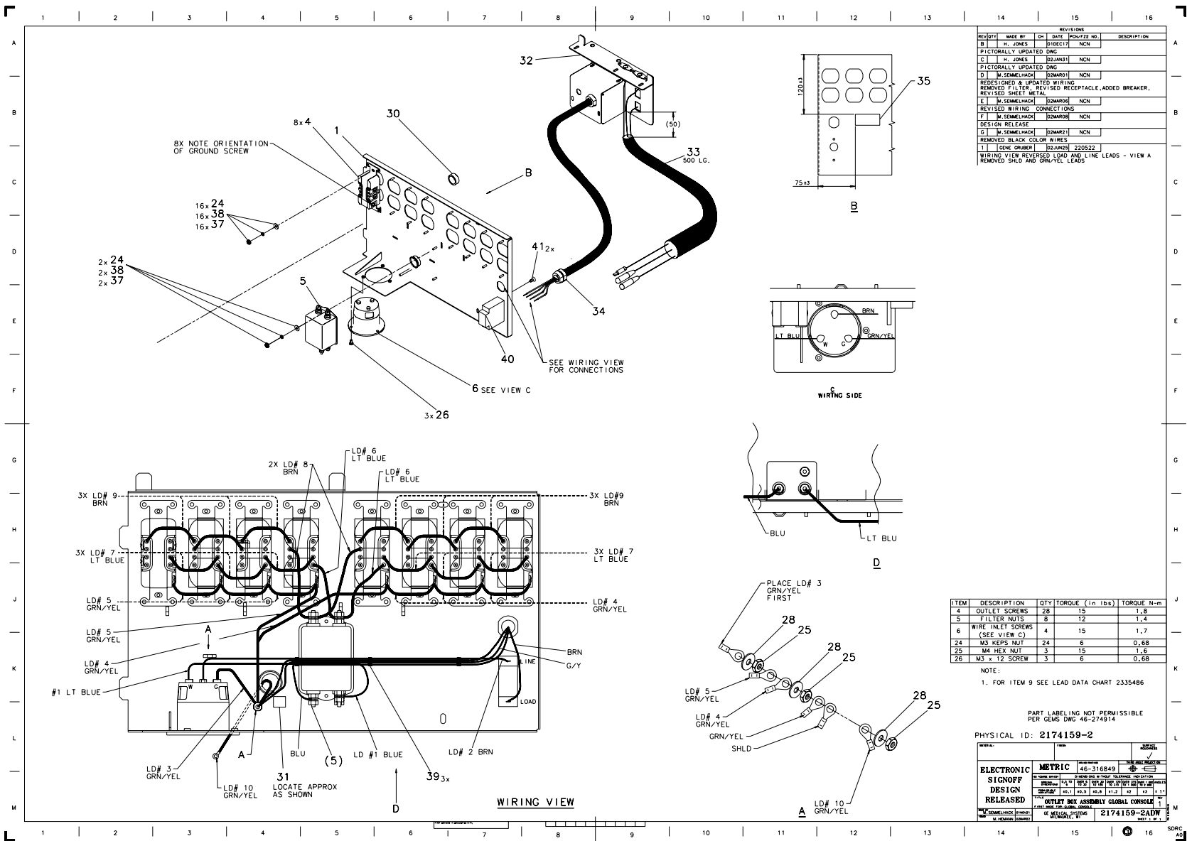
Figure 7-23 Outlet Box Assembly (2174159-2, sheet 1, rev 1)
