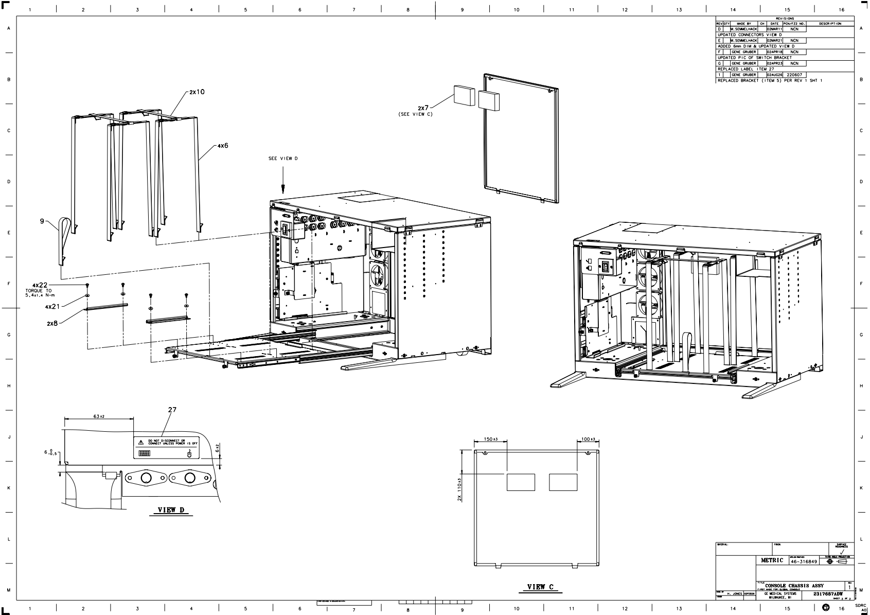
Figure 7-27 Console Chassis Assembly (2317687, sheet 2, rev 1)
