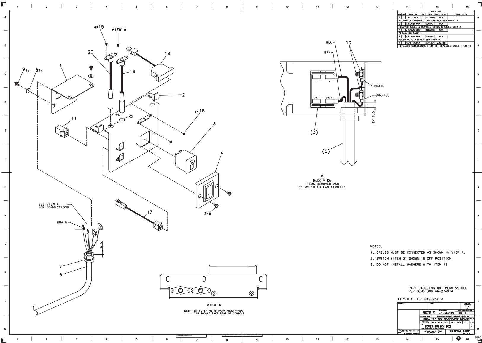
Figure 7-24 Power Switch Box (2190750-2, sheet 1, rev 1)
