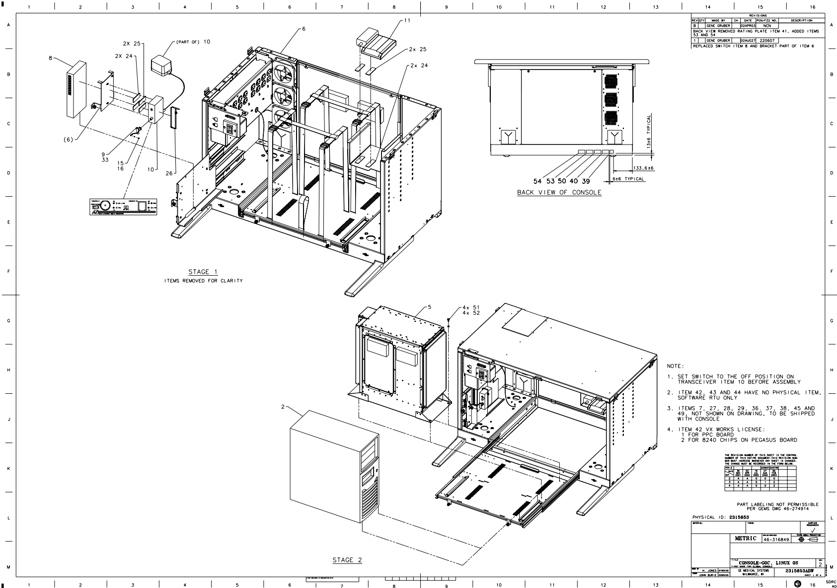
Figure 7-3 Console Assembly (2315653, sheet 1, rev 2)
