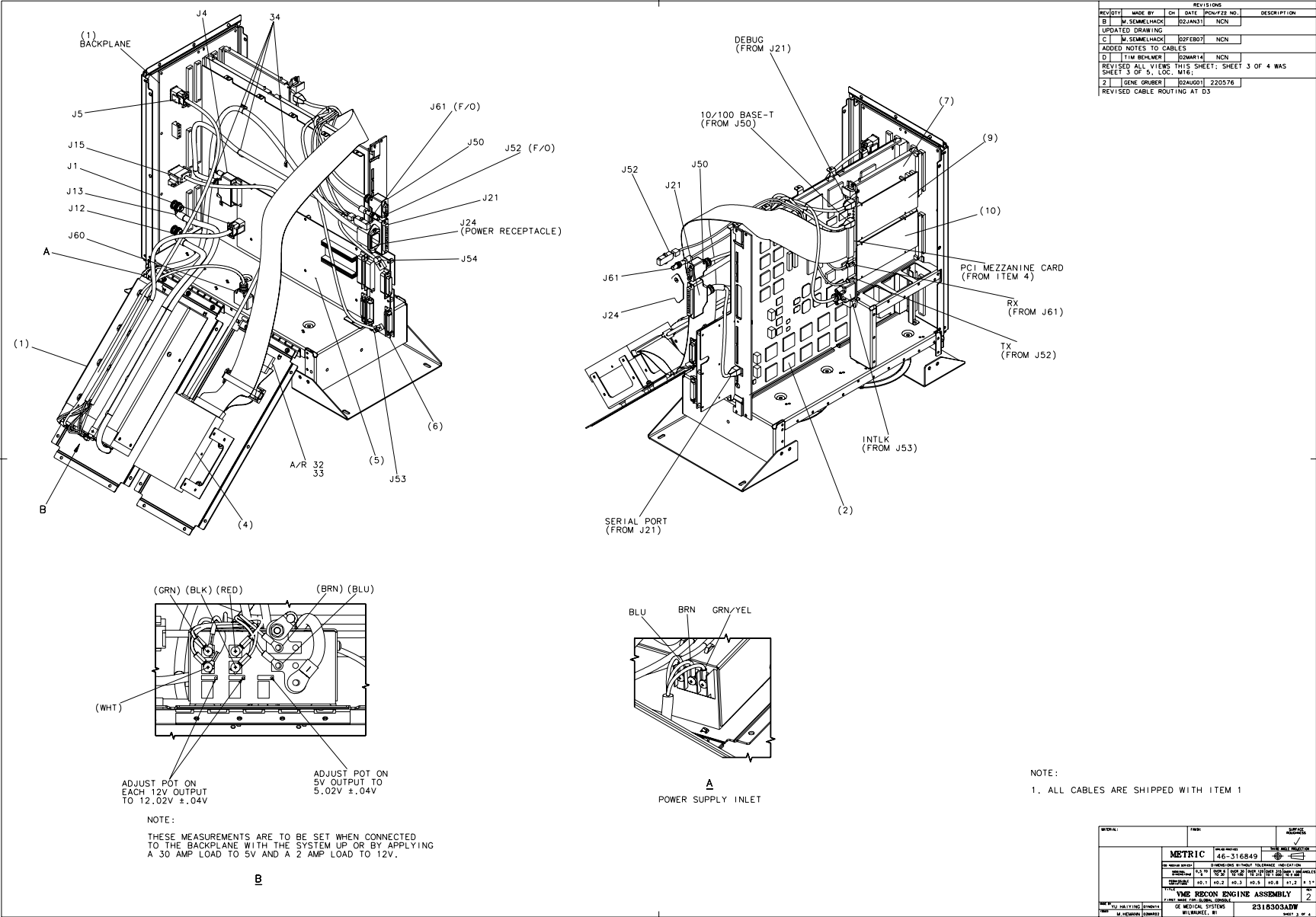
Figure 7-11 VME Recon Engine Assembly (2318303, sheet 3, rev 2)
