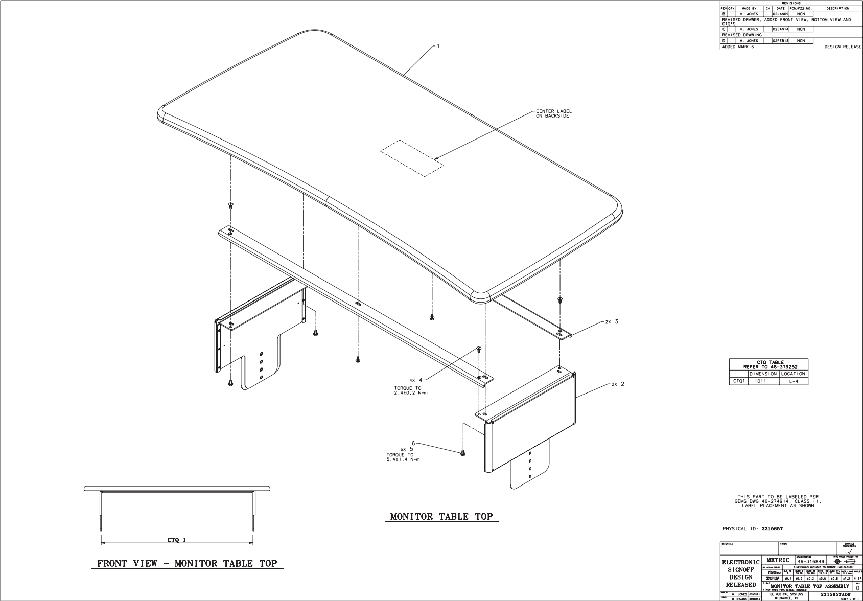
Figure 7-7 Table Top Assembly, Monitor (2315657, sheet 1, rev 0)
