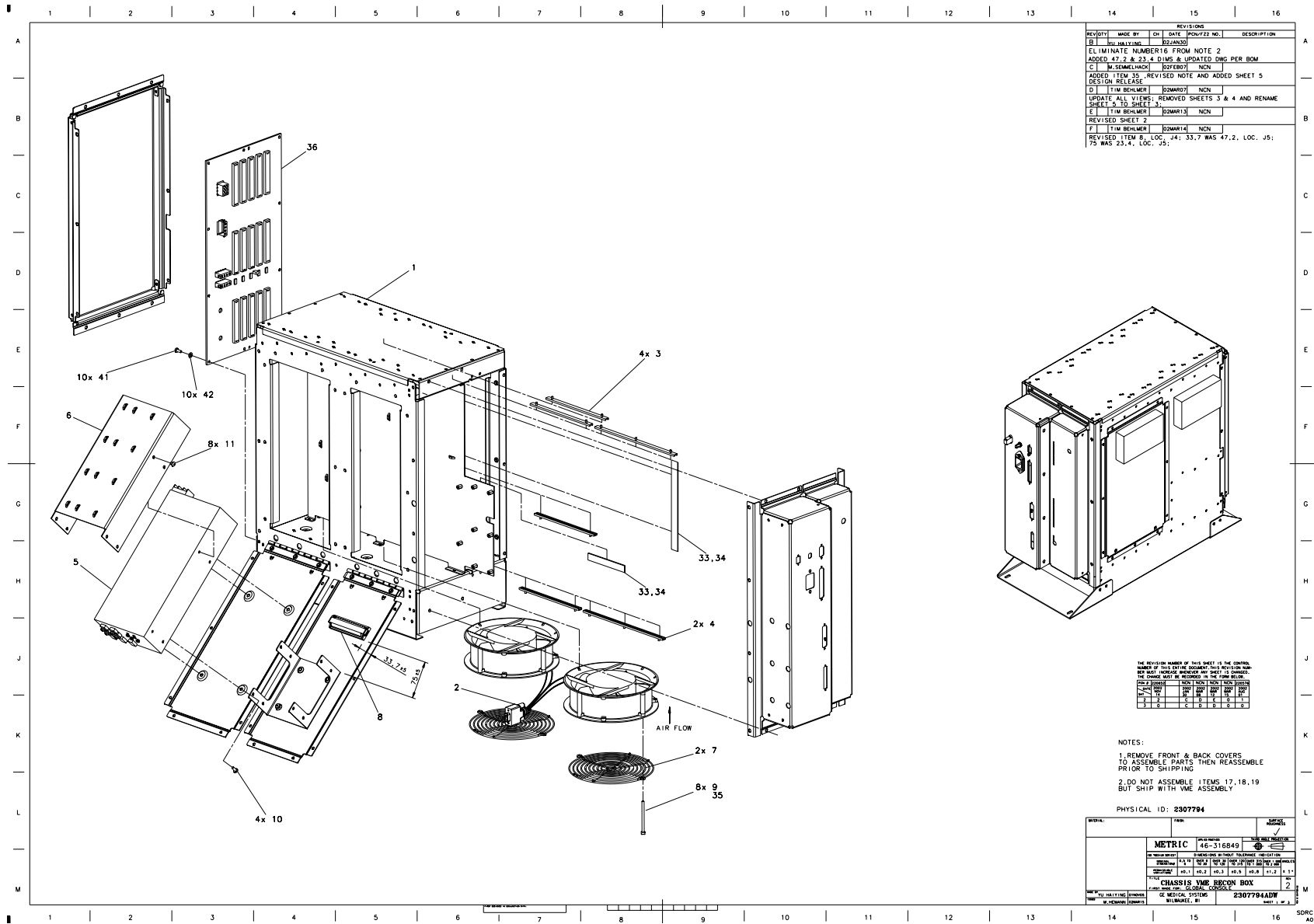
Figure 7-18 VME Chassis Assembly (2307794, sheet 1, rev 2)
