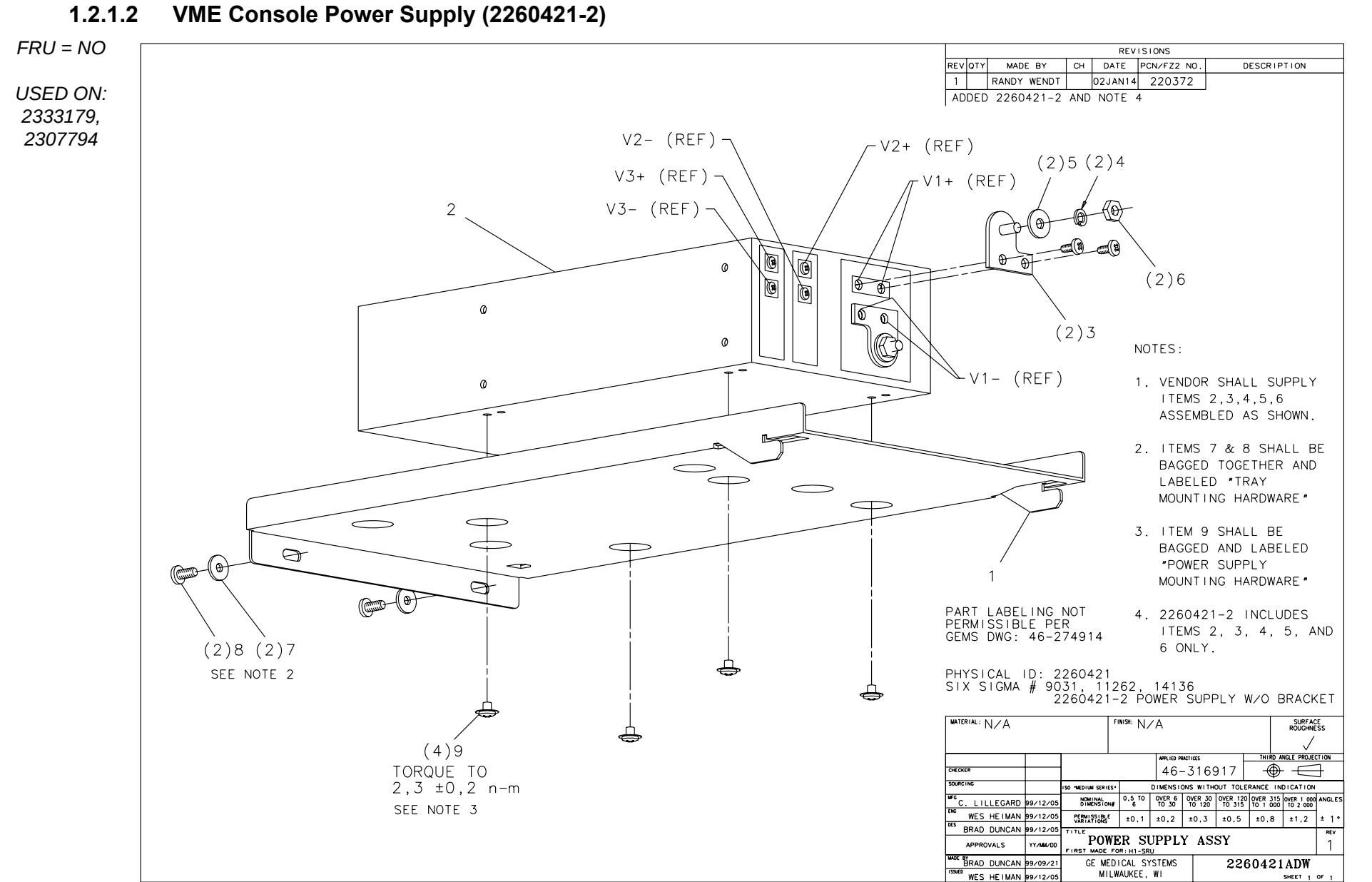
Figure 7-17 VME Console Power Supply (2260421, sheet 1, rev 1)
