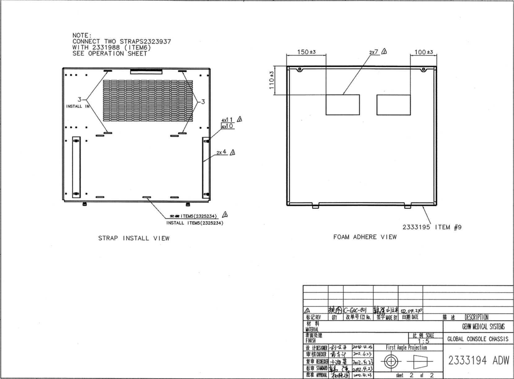
Figure 7-22 Console Chassis Assembly (2333194 sheet 2, rev 1)
