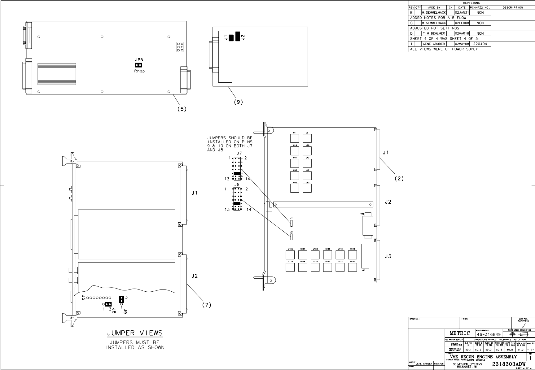
Figure 7-12 VME Recon Engine Assembly (2318303, sheet 4, rev 1)
