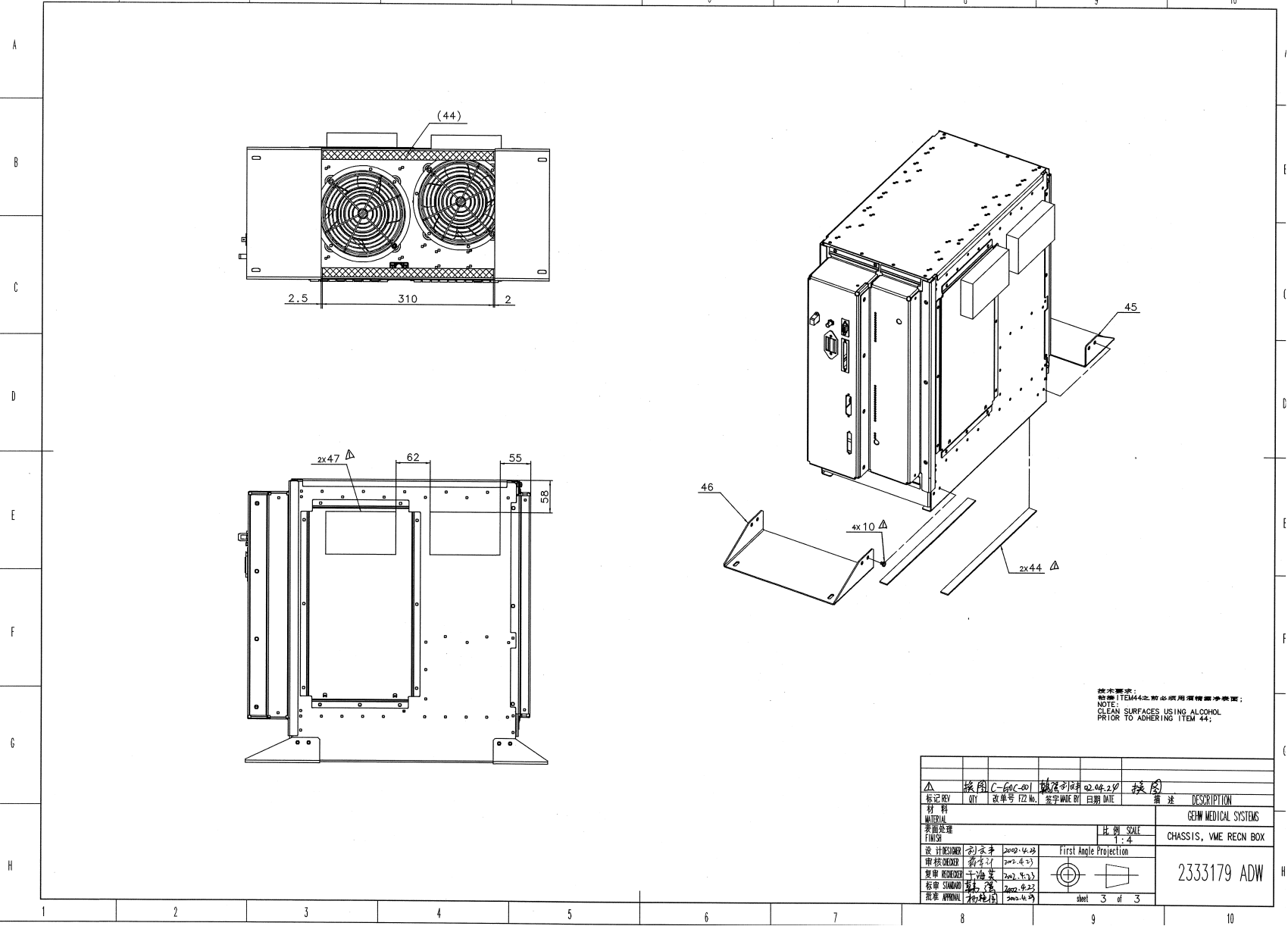
Figure 7-15 Chassis, VME Recon Box (2333179 sheet 3, rev 1)
