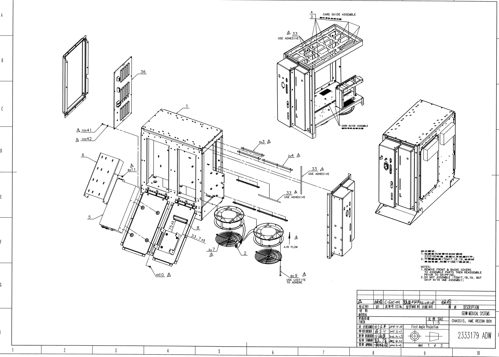
Figure 7-13 Chassis, VME Recon Box (2333179 sheet 1, rev 1)
