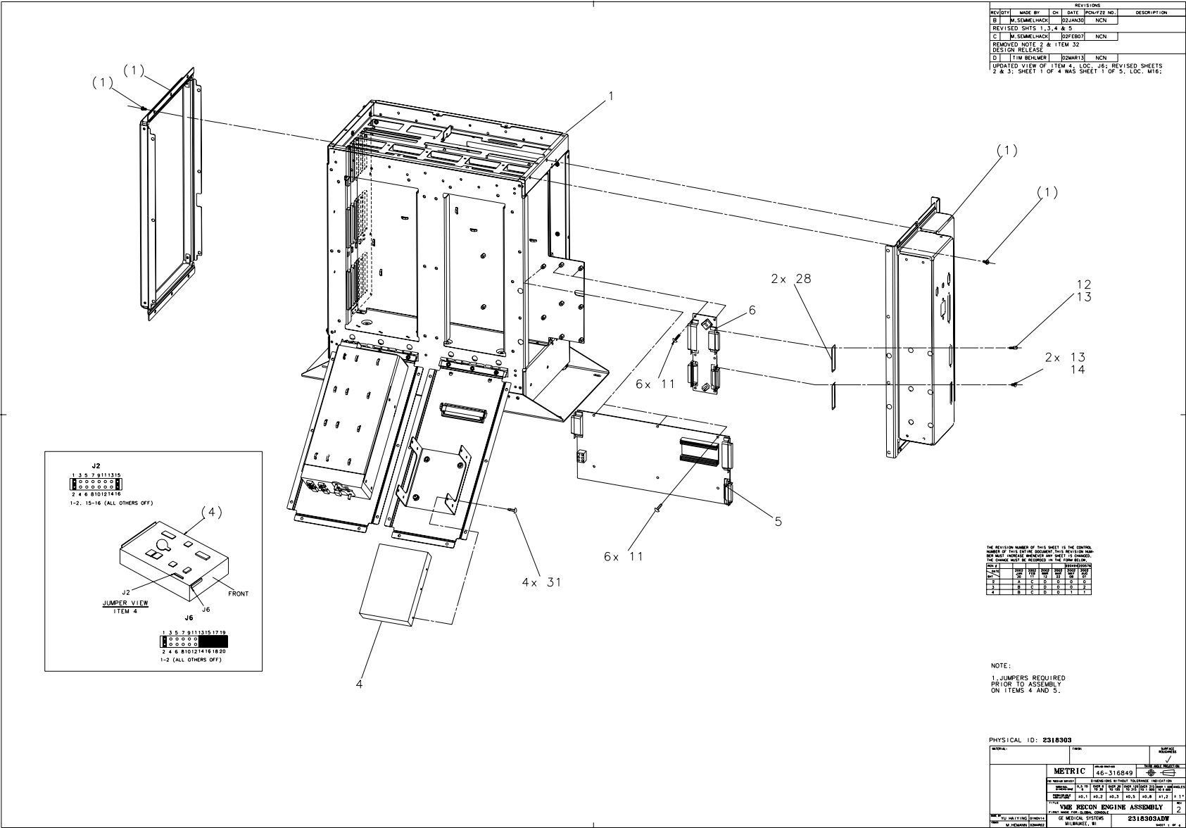
Figure 7-9 VME Recon Engine Assembly (2318303, sheet 1, rev 2)
